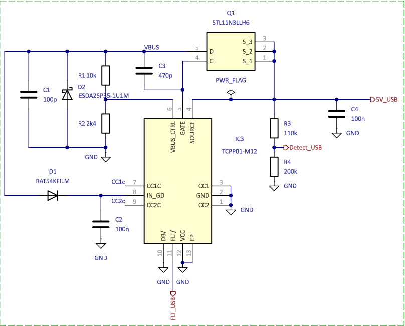
USB-C power sink, 5V, 15W
