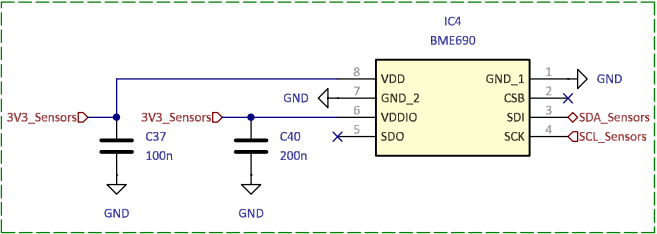
Pressure and temperature sensor
