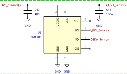
Humidity sensor
