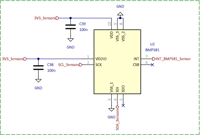
Pressure and temperature sensor
