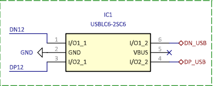
ESD protection on USB-C data lines
