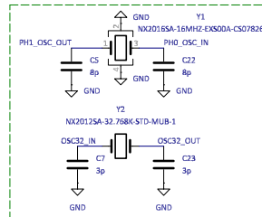
Crystal oscillators (HSE and LSE)
