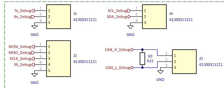
Communication interface connectors
