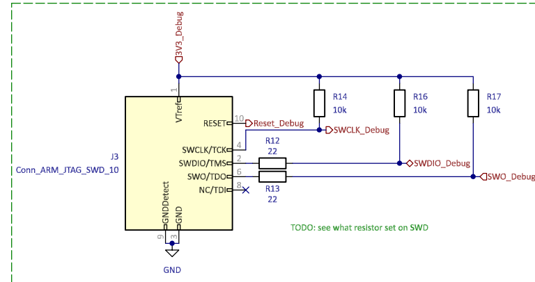
Communication interface connectors
