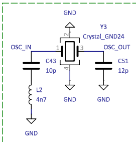
Crystal oscillator
