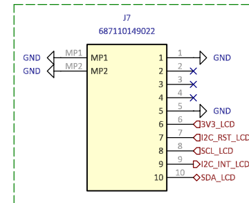
TFT LCD 10 pins touch connector
