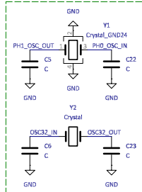
Crystal oscillators (HSE and LSE)
