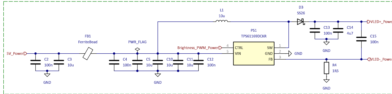
LED driver
