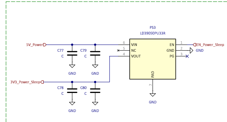
LDO 5V -> 3.3V
