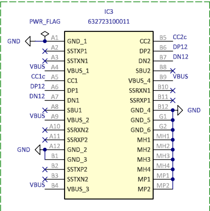
USB-C connector right angle
