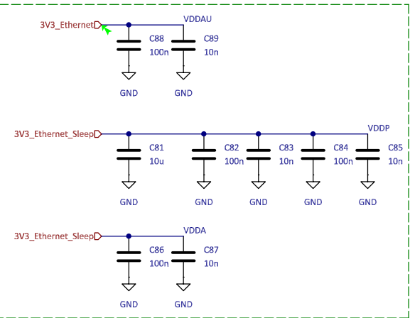
Ethernet LAN8651 decoupling capacitors
