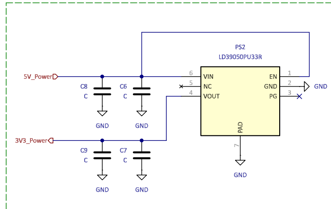
LDO 5V -> 3.3V
