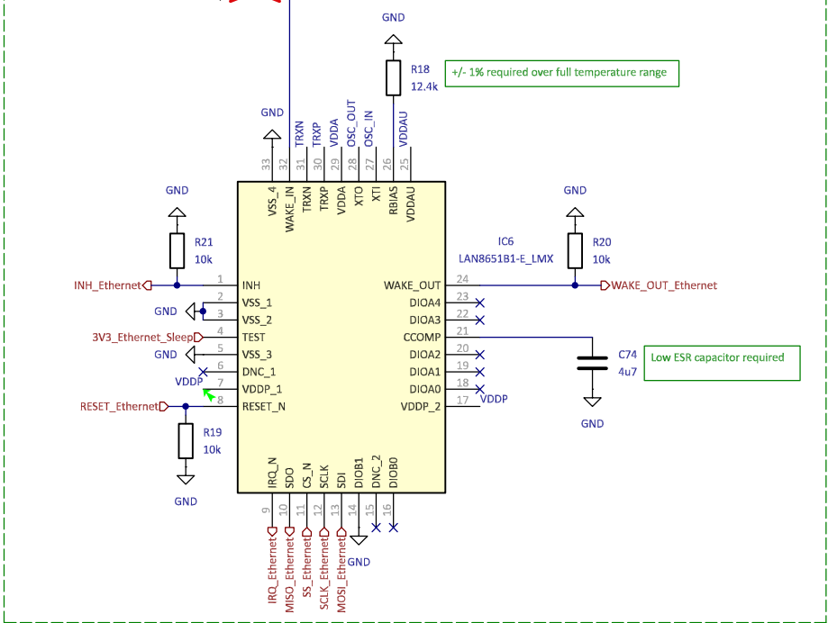
External Ethernet PHY
