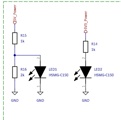
LED driver
