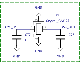
LAN8651 25MHz oscillator
