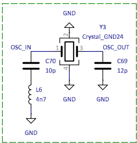
Crystal oscillator
