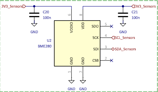
Humidity sensor
