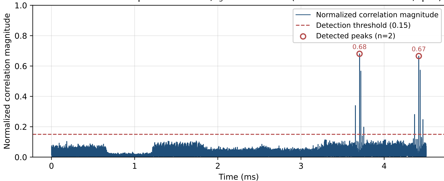
ZC matched-filter output — root 147, f_s = 50.00 MHz (decimated to 16.67 MHz, q=3 )
