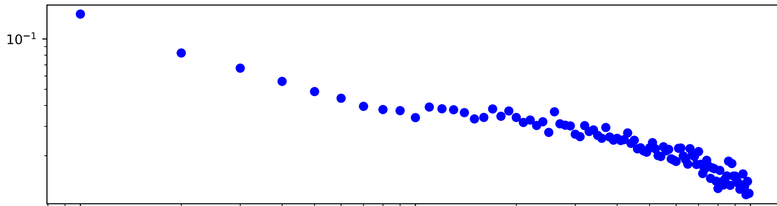
Trade sign correlation function
