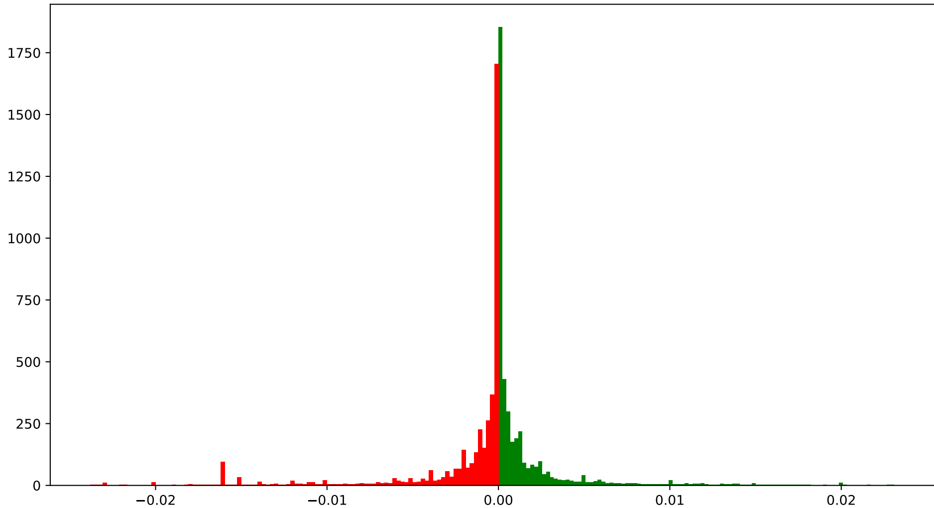
Histogram of trades between 2025-11-20 and 2025-11-24
