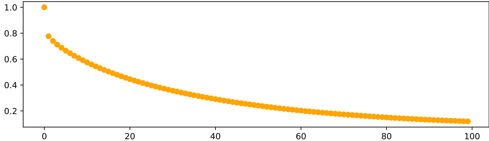
Trade sign correlation function
