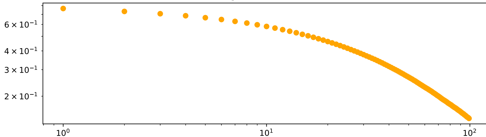
Trade sign correlation function
