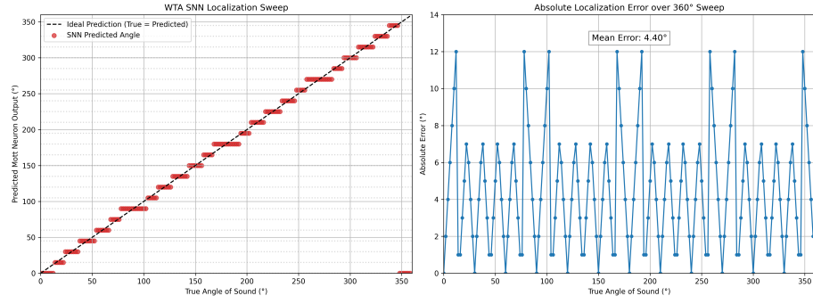
Figure 4: Localization accuracy evaluated across a full 360^\circ sweep using the optimized LIF parameters in the ideal acoustic simulation.
