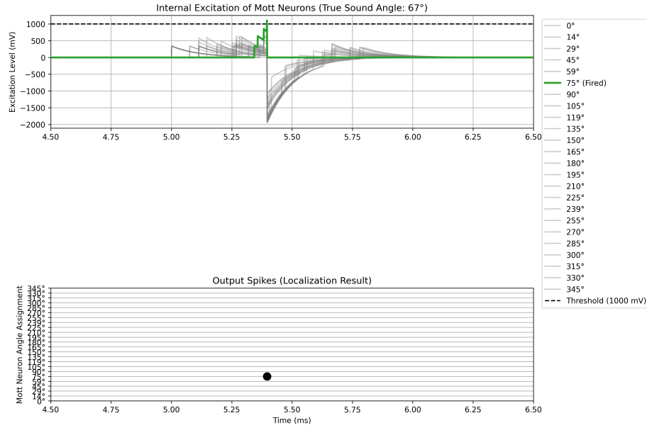
Figure 2: Ideal acoustic simulation of a sound wave arriving from 67° and the corresponding sub-threshold voltage traces of the Mott neurons.
