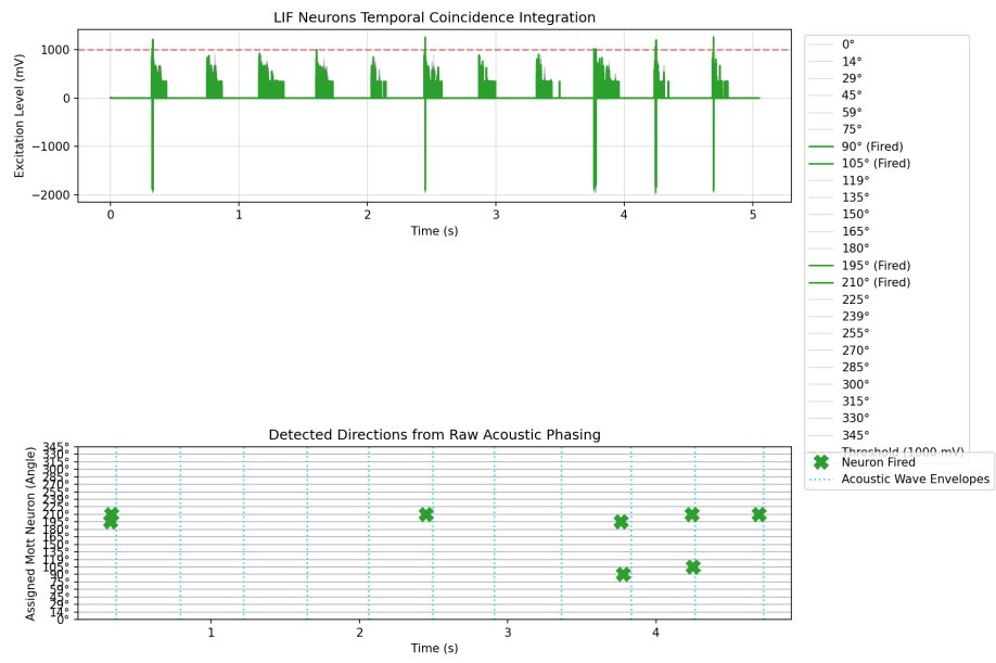
Figure 5: Predicting the DoA with coincidence detection simulation. The sound source was clapping.
