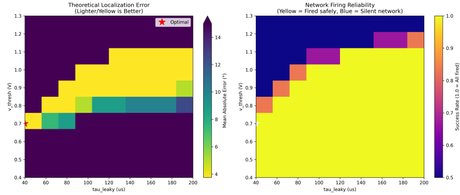
Figure 3: Parameter optimization grid search mapping the theoretical localization error limits, demonstrating the optimal parameter selection.
