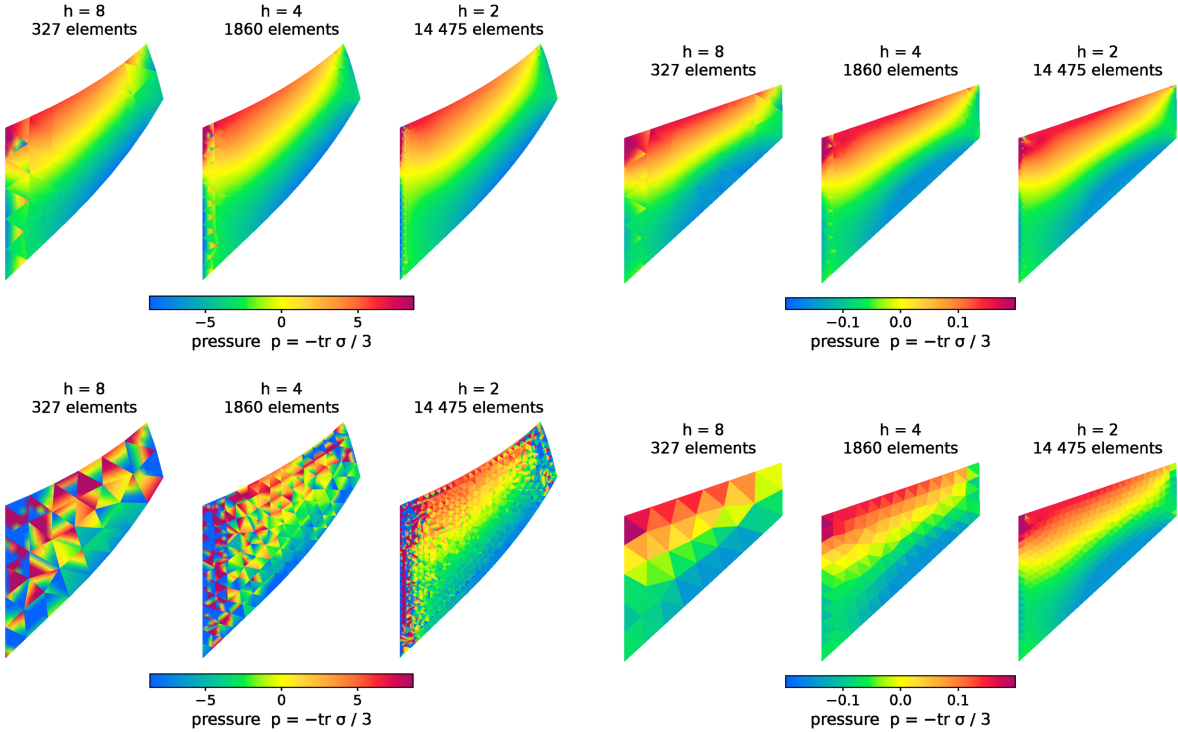
Figure 3: Pressure on the face z = 10 under mesh refinement, h = 8, 4, 2 from left to right in each panel, with the color scale of the case. Top: TETRA15 with the linear projection, elastic (left) and plastic (right). Bottom left: TETRA10 pointwise, elastic. Bottom right: the composite tetrahedron, plastic.
