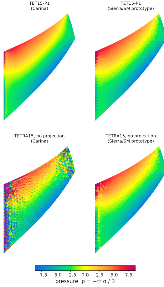
Figure 4: Cook's membrane, elastic case, h = 2 : pressure on the front face at full load, on the color scale of Figure 1. Top, TET15-P1 in Carina (the quadratic of each element) and in a prototype implementation in Sierra/SM (one value per element); bottom, TETRA15 without the projection in the two codes.
