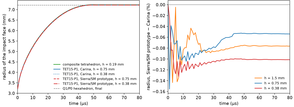
Figure 6: Taylor bar: TET15-P1 in Carina and in a prototype implementation in Sierra/SM on the same meshes. Left, the radius of the impact face against time, with the composite tetrahedron at h = 0.19 mm; right, the relative difference of the two codes’ radii at every level.
