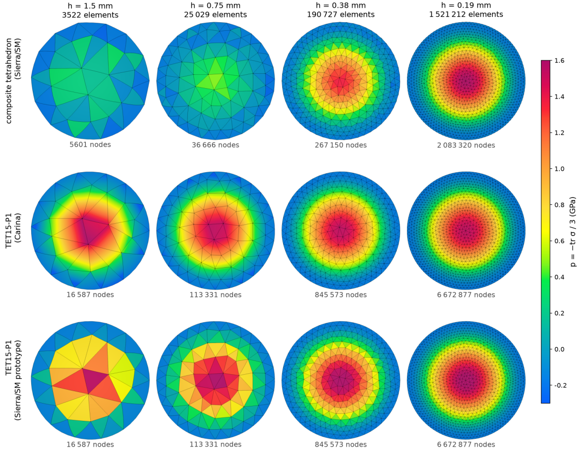
Figure 7: Taylor bar: pressure on the impact face at 12\mu\text{s} on the scale of Figure 8, for the composite tetrahedron (Sierra/SM), TET15-P1 in Carina and TET15-P1 in a prototype implementation in Sierra/SM (one value per element).
