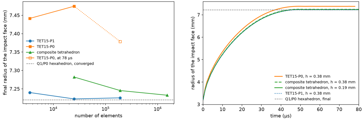
Figure 5: Taylor bar. Left: final radius of the impact face against the number of elements; the open square is TET15-P0 at 78\mu\text{s} . Right: radius of the impact face against time for TET15-P1 and TET15-P0 at h = 0.38 mm and the composite tetrahedron at h = 0.38 and 0.19 mm. Dashed gray: the converged Q1/P0 hexahedron of Foulk III et al. [14]. Script: benchmark/tet15-p1/taylor/plot.py .
