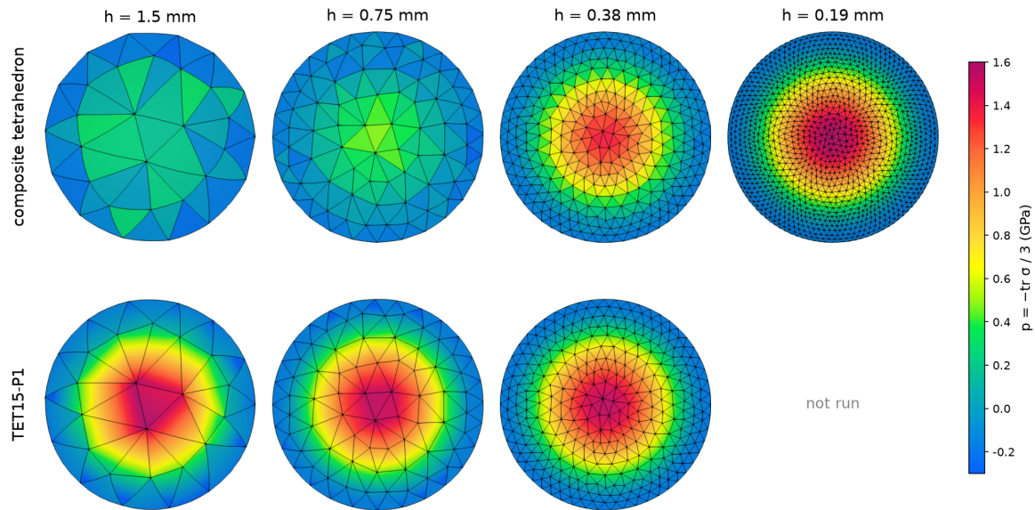
Figure 5: Taylor bar, pressure p = -\frac{1}{3} \text{tr } \boldsymbol{\sigma} on the impact face at t = 12\mu\text{s} , seen along the axis, on the same meshes for both elements; one color scale, values beyond it saturate. Top: composite tetrahedron (Sierra/SM, \alpha = 0.1 , exponent 0), one value per element. Bottom: TET15-P1, the quadratic fitted in each element; not run at h = 0.19 mm.
