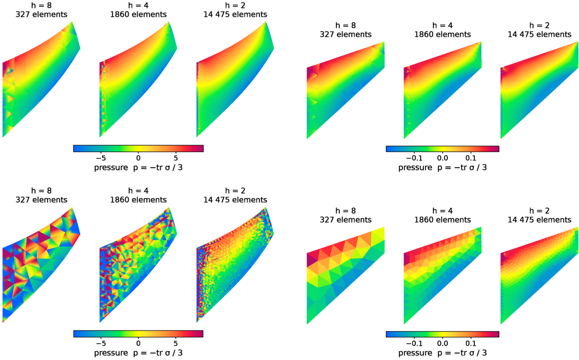
Figure 3: Pressure on the face z = 10 under mesh refinement, h = 8, 4, 2 from left to right in each panel, with the color scale of the case. Top: TETRA15 with the linear projection, elastic (left) and plastic (right). Bottom left: TETRA10 pointwise, elastic. Bottom right: the composite tetrahedron, plastic.
