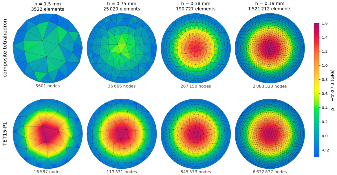
Figure 5: Taylor bar, pressure p = -\frac{1}{3} \text{tr } \sigma on the impact face at t = 12\mu\text{s} , seen along the axis, on the same meshes for both elements, with the element count of each level and the node count of each mesh (TETRA10 for the composite tetrahedron, TETRA15 for TET15-P1); one color scale, values beyond it saturate. Top: composite tetrahedron (Sierra/SM, \alpha = 0.1 , exponent 0), one value per element. Bottom: TET15-P1, the quadratic fitted in each element.
