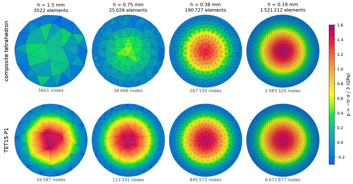
Figure 5: Taylor bar, pressure p = -\frac{1}{3} \text{tr } \boldsymbol{\sigma} on the impact face at t = 12\mu\text{s} , seen along the axis, on the same meshes for both elements, with the element count of each level and the node count of each mesh ( TETRA10 for the composite tetrahedron, TETRA15 for TET15-P1); one color scale, values beyond it saturate. Top: composite tetrahedron (Sierra/SM, \alpha = 0.1 , exponent 0), one value per element. Bottom: TET15-P1, the quadratic fitted in each element.
