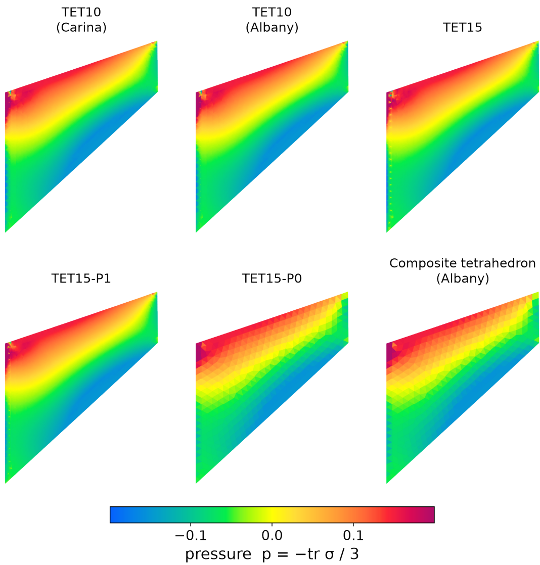
Figure 2: Plastic case, h = 2 : pressure on the face z = 10 at full load, as in Figure 1.
