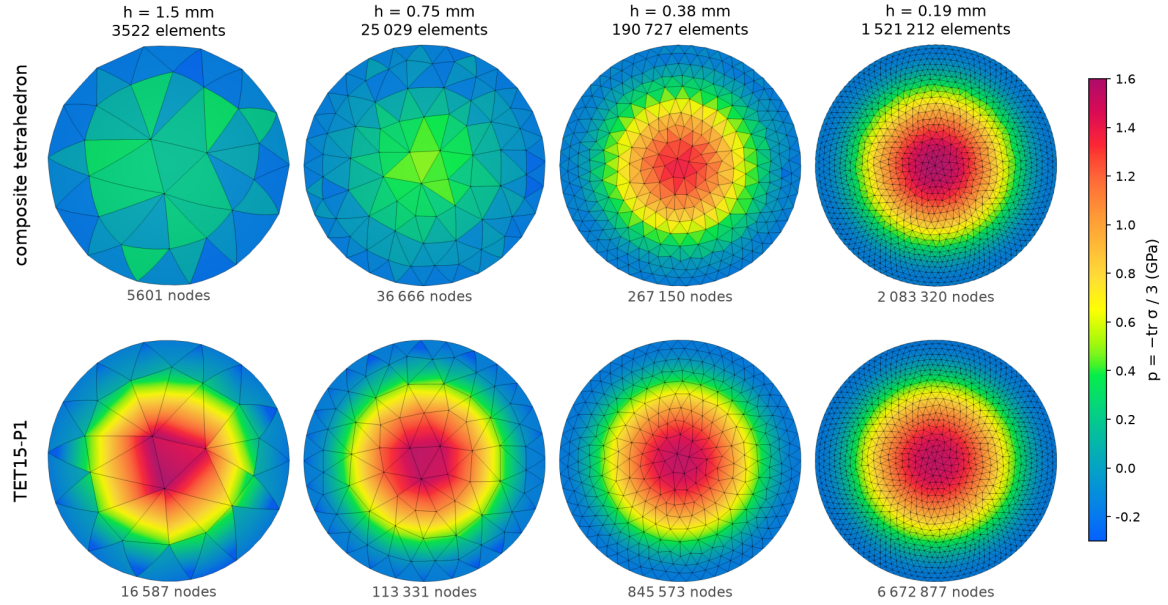
Figure 6: Taylor bar, pressure p = -\frac{1}{3} \text{tr } \boldsymbol{\sigma} on the impact face at t = 12 \mu\text{s} , seen along the axis, on the same meshes for both elements, with the element count of each level and the node count of each mesh (TETRA10 for the composite tetrahedron, TETRA15 for TET15-P1); one color scale, values beyond it saturate. Top: composite tetrahedron (Sierra/SM, \alpha = 0.1 , exponent 0), one value per element. Bottom: TET15-P1, the quadratic fitted in each element.
