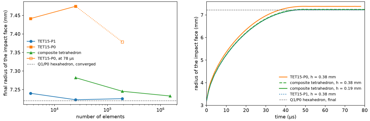
Figure 4: Taylor bar. Left: final radius of the impact face against the number of elements; the open square is TET15-P0 at 78\mu\text{s} . Right: radius of the impact face against time for TET15-P1 and TET15-P0 at h = 0.38 mm and the composite tetrahedron at h = 0.38 and 0.19 mm. Dashed gray: the converged Q1/P0 hexahedron of Foulk III et al. [14]. Script: benchmark/tet15-p1/taylor/plot.py .
