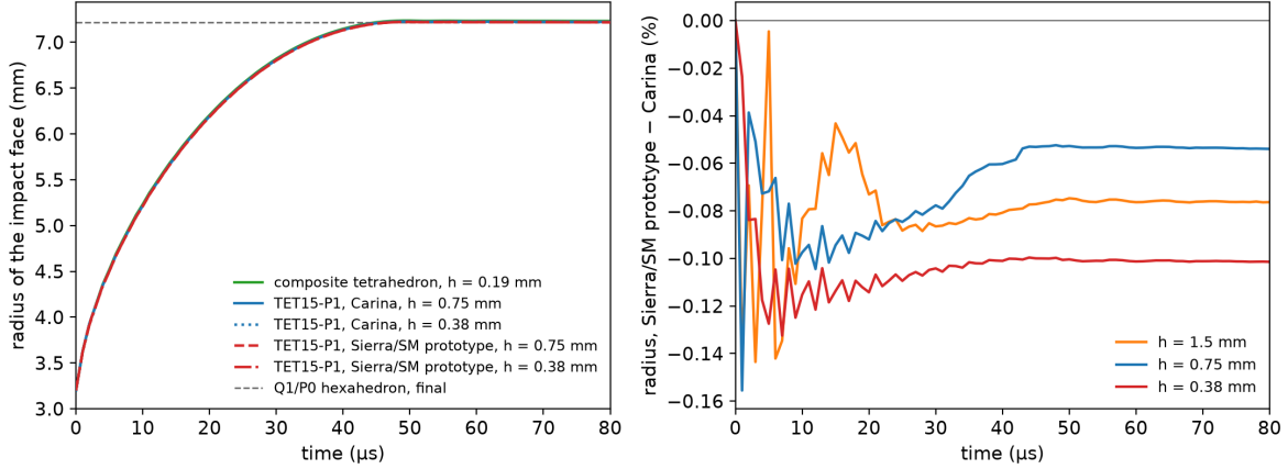
Figure 5: Taylor bar: TET15-P1 in Carina and in a prototype implementation in Sierra/SM on the same meshes. Left, the radius of the impact face against time, with the composite tetrahedron at h = 0.19 mm; right, the relative difference of the two codes’ radii at every level.
