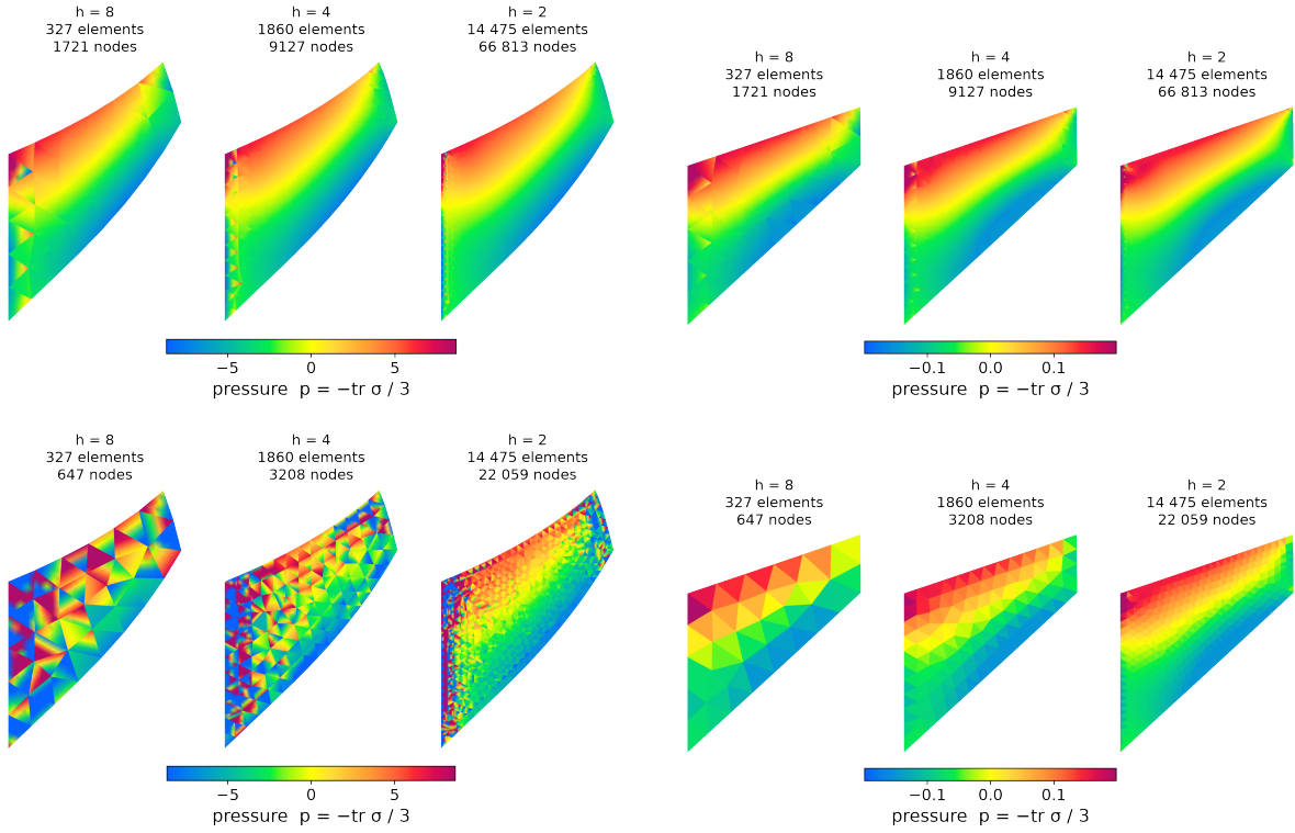
Figure 3: Pressure on the face z = 10 under mesh refinement, h = 8, 4, 2 from left to right in each panel, with the color scale of the case. Top: TET15-P1, elastic (left) and plastic (right). Bottom left: TET10 pointwise, elastic. Bottom right: the composite tetrahedron, plastic.
