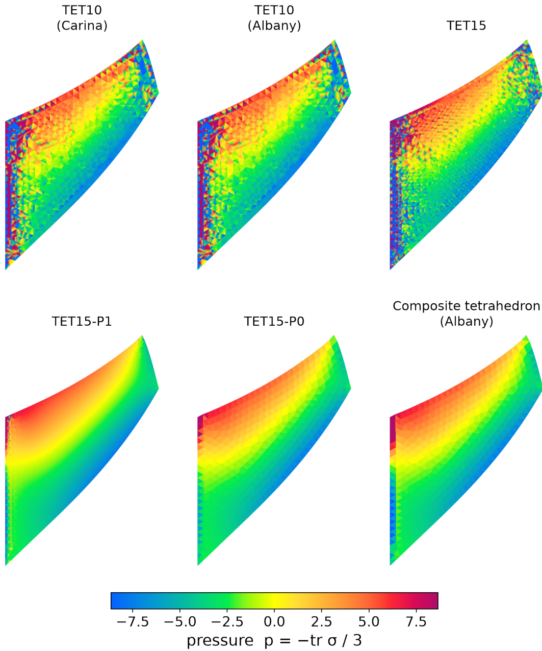
Figure 1: Elastic case, h = 2 : pressure p = -\text{tr } \sigma / 3 on the face z = 10 of the deformed membrane at full load, for the six elements. One color scale for all panels, symmetric about zero and bounded by the 99th percentile of |p| over TET15-P1, TET15-P0 and the composite tetrahedron; values beyond the scale saturate. Inside each element the pressure drawn is the polynomial fitted to the quadrature-point values (text).
