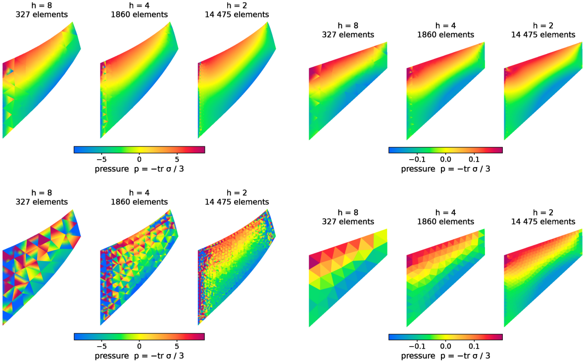
Figure 3: Pressure on the face z = 10 under mesh refinement, h = 8, 4, 2 from left to right in each panel, with the color scale of the case. Top: TET15-P1, elastic (left) and plastic (right). Bottom left: TET10 pointwise, elastic. Bottom right: the composite tetrahedron, plastic.
