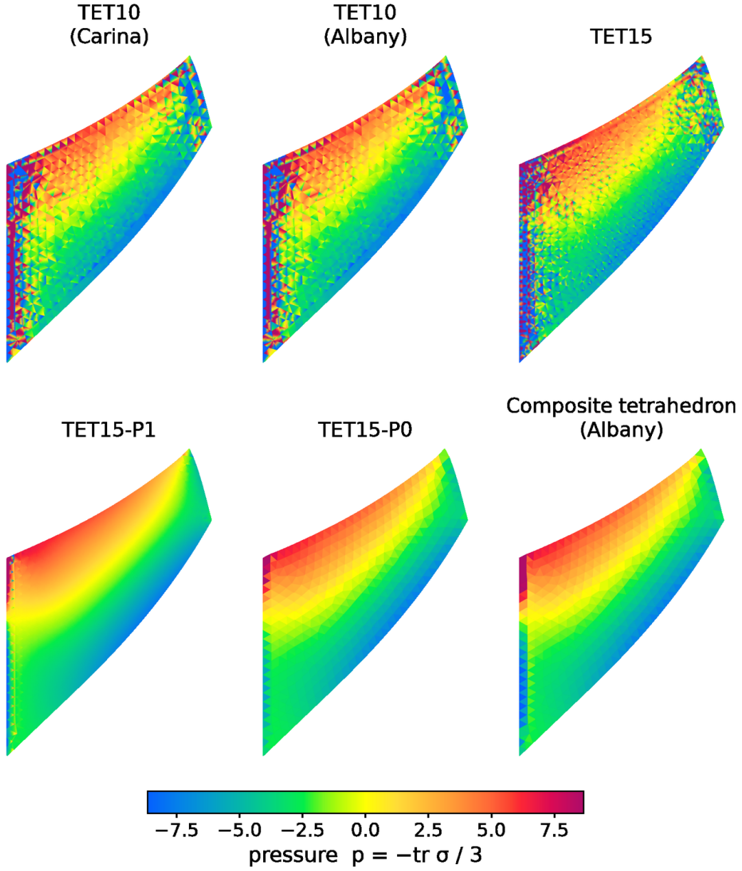
Figure 1: Elastic case, h = 2 : pressure p = -\text{tr } \boldsymbol{\sigma} / 3 on the face z = 10 of the deformed membrane at full load, for the six elements. One color scale for all panels, symmetric about zero and bounded by the 99th percentile of |p| over TET15-P1, TET15-P0 and the composite tetrahedron; values beyond the scale saturate. Inside each element the pressure drawn is the polynomial fitted to the quadrature-point values (text).
