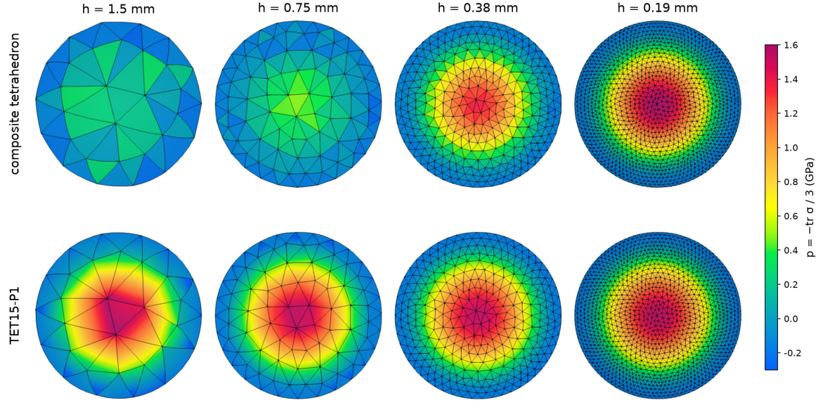
Figure 5: Taylor bar, pressure p = -\frac{1}{3} \text{tr } \boldsymbol{\sigma} on the impact face at t = 12 \mu\text{s} , seen along the axis, on the same meshes for both elements; one color scale, values beyond it saturate. Top: composite tetrahedron (Sierra/SM, \alpha = 0.1 , exponent 0), one value per element. Bottom: TET15-P1, the quadratic fitted in each element.
