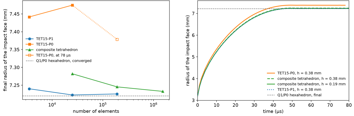
Figure 4: Taylor bar. Left: final radius of the impact face against the number of elements; the open square is TET15-P0 at 78 \mu s. Right: radius of the impact face against time for TET15-P1 and TET15-P0 at h = 0.38 mm and the composite tetrahedron at h = 0.38 and 0.19 mm. Dashed gray: the converged Q1/P0 hexahedron of Foulk III et al. [14]. Script: benchmark/tet15-p1/taylor/plot.py .
