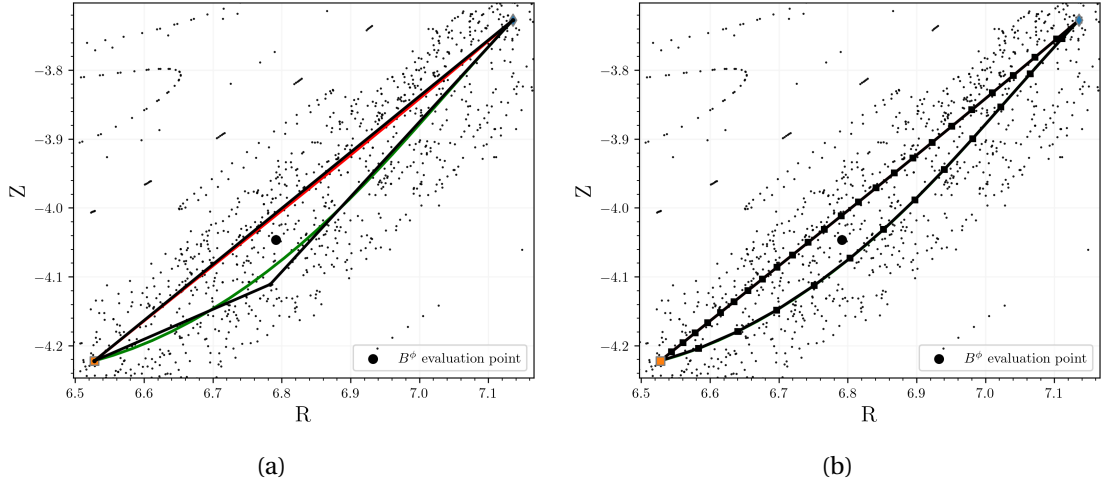
Figure 3.8: Surface and evaluation point for the approximation of the flux through the lobe. In (a) a simple triangle is considered and in (b) the boundary of \Sigma_{lobe} is found by tracing points in W^s and W^u . The B^\phi component of the magnetic field is evaluated at a random inner point of the lobe.
