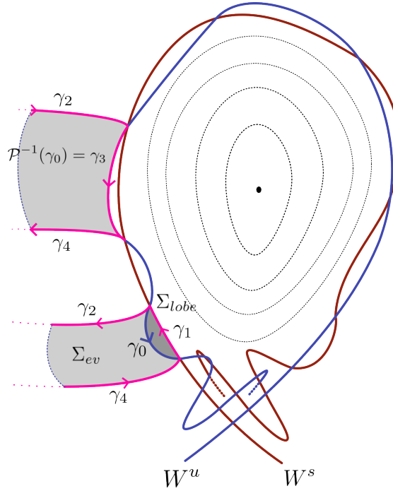
Figure 3.4: Schematic representation of the calculation of the turnstile area in a homoclinic tangle. The tangle is formed by W^s and W^u in a chaotic configuration of the Toy-Tokamak with perturbation m/n = 6/1 . A turnstile lobe is depicted as \Sigma_{lobe} with boundary \gamma_0 + \gamma_1 and the boundary of a more complex surface with identical flux \Sigma = \Sigma_{lobe} + \Sigma_{ev} is especially emphasised in pink.
