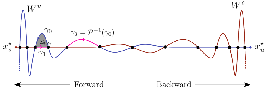
Figure 3.5: Flatten out version of the manifold tangle structure between two saddle fixed points x_s^* and x_u^* . The forward evolution \mathcal{P} maps points close to x_u^* in the direction of x_s^* and the backward evolution the opposite. Two different hetero/homo-clinics are present and are denoted by the squared and circular markers. The surface of the lobe \Sigma_{lobe} , as well as the joining curves \gamma_1 and \gamma_3 are highlighted.
