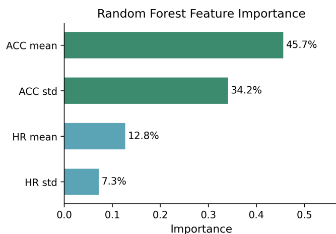
Figure 2: Random Forest feature importance for the 2-class activity classifier. Accelerometer features (ACC) account for 79.9% of importance, confirming movement as the primary distinguisher between physical activity and cognitive states.
