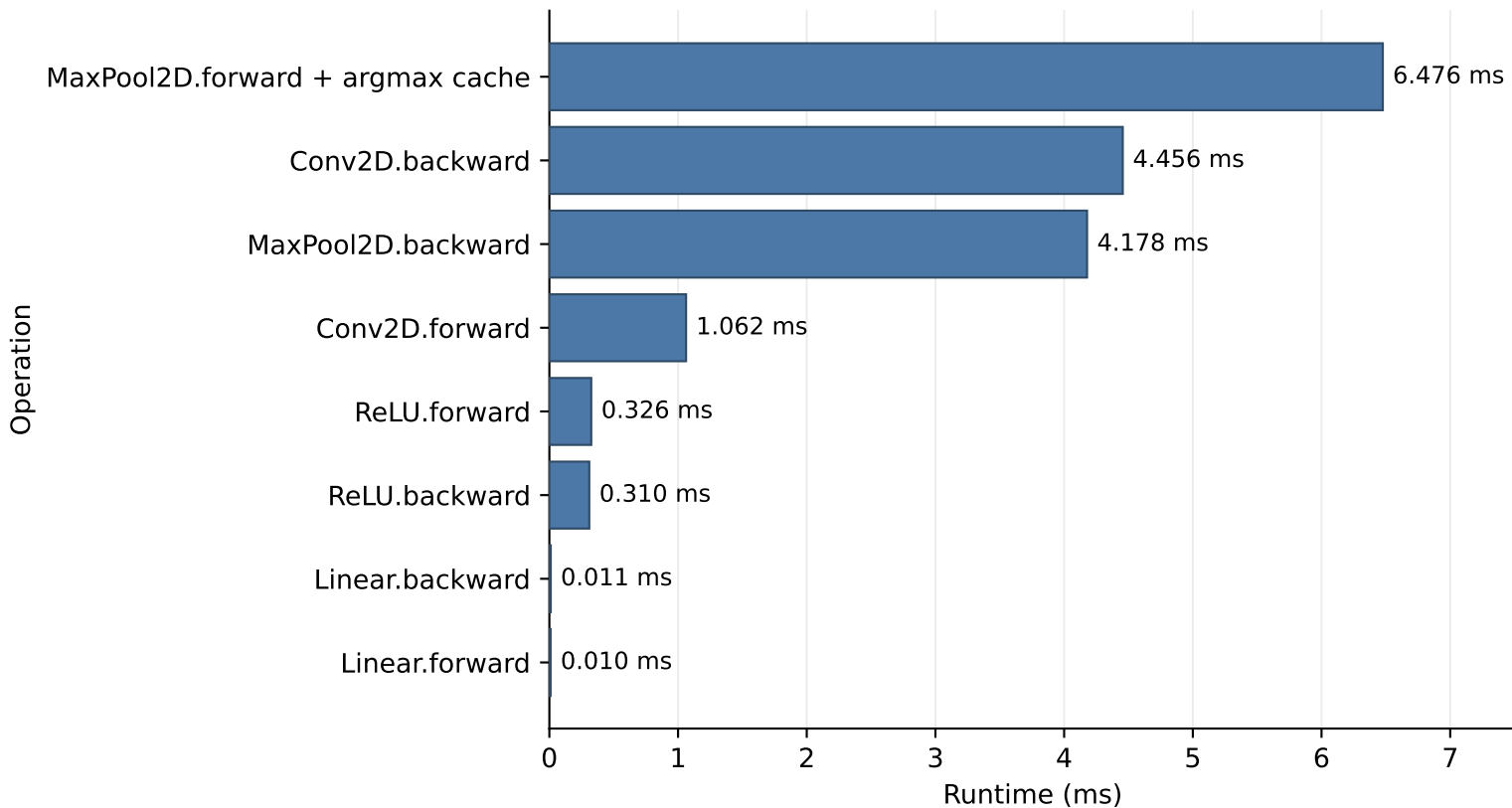
Runtime Breakdown of Core CNN Operations
