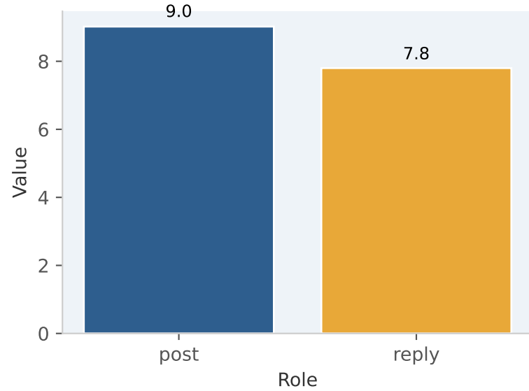
% Messages with '?'
