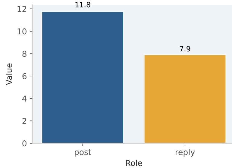
% Messages with '?'
