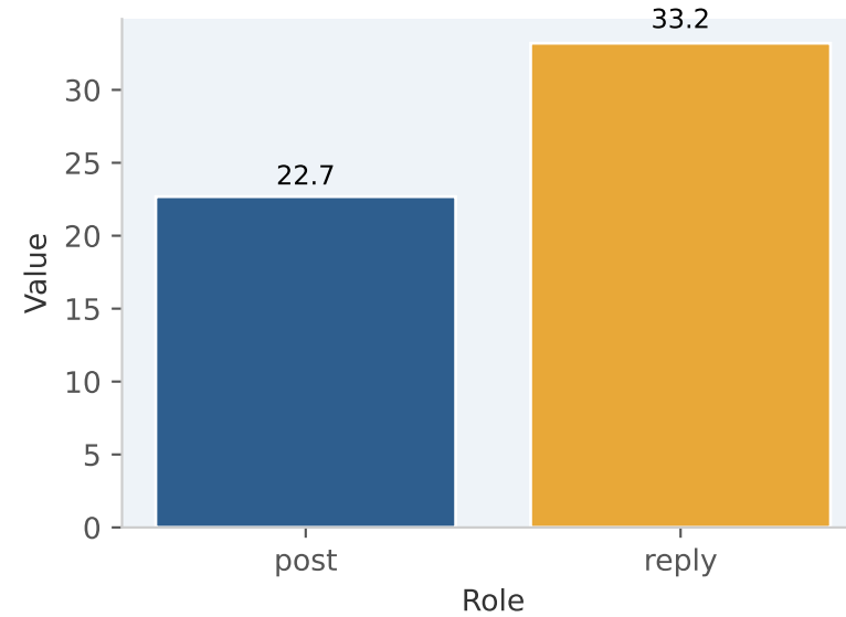
% Messages with '!'
