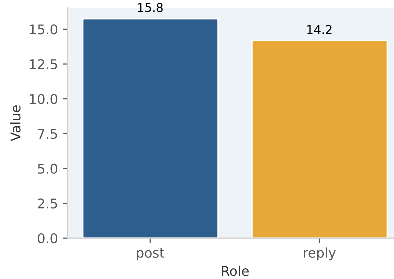
% Messages with '!'
