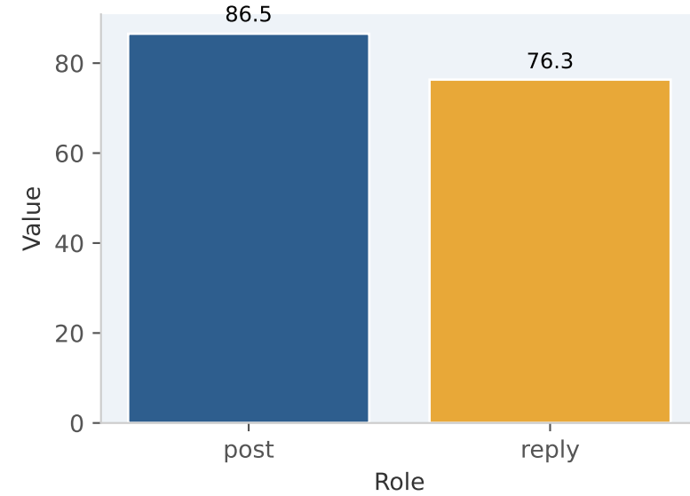
% Messages with '...'
