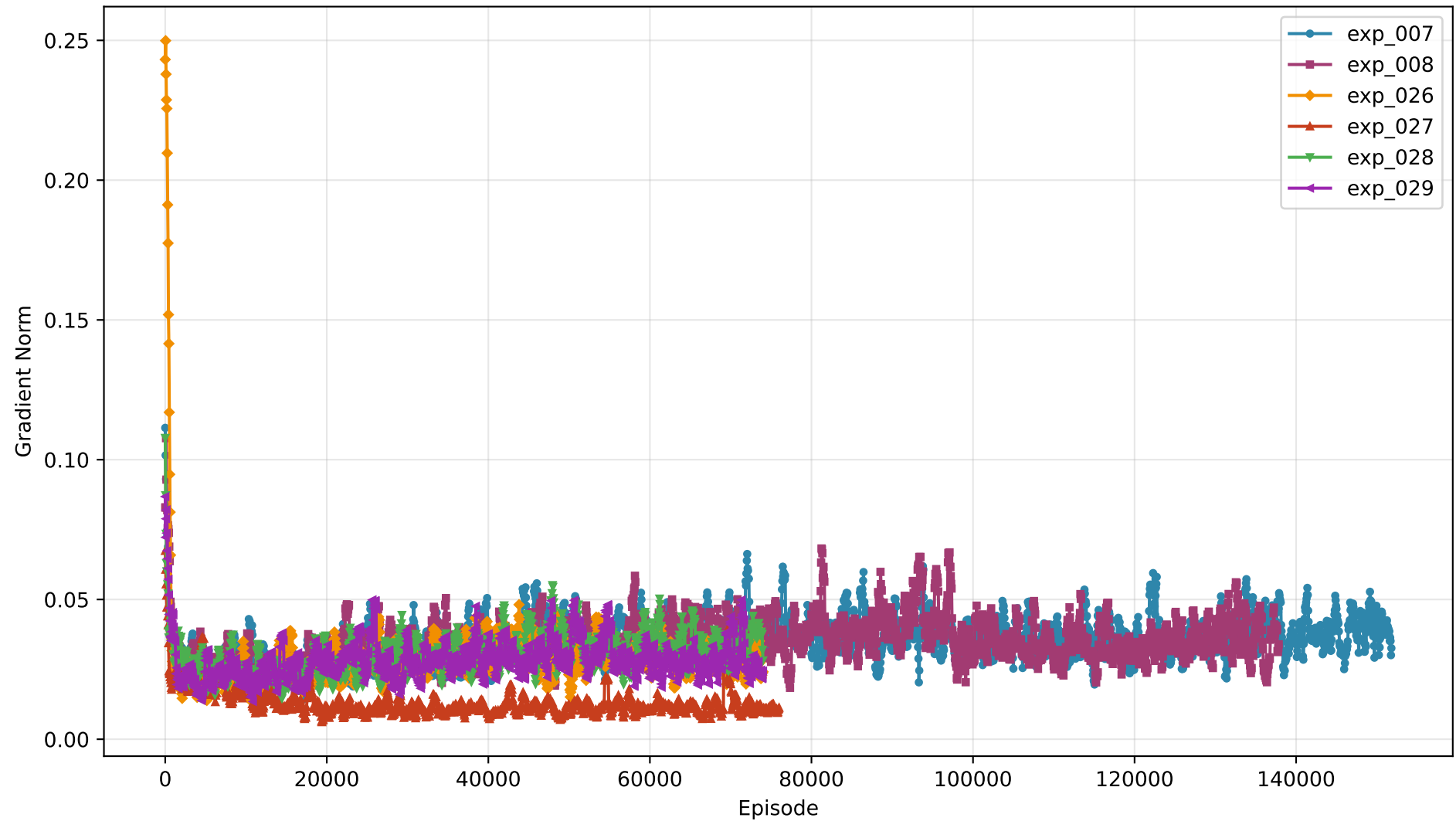
Gradient Norm vs Episode
