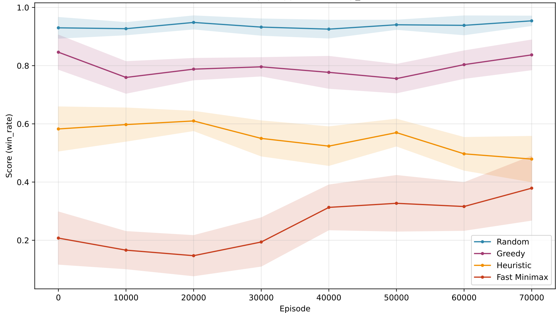
Win Rate per Opponent — exp_029
