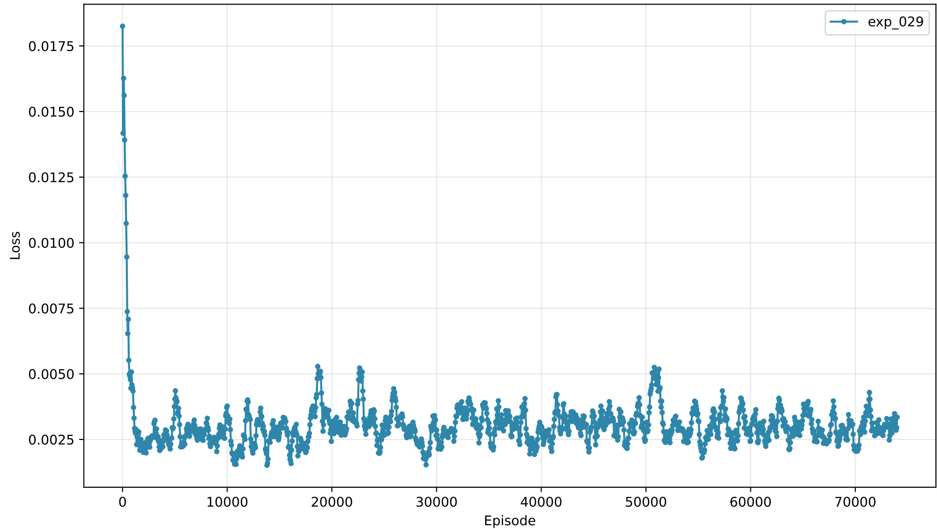
Loss vs Episode
