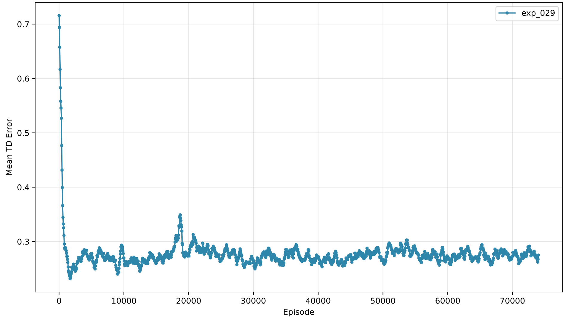
Mean TD Error vs Episode
