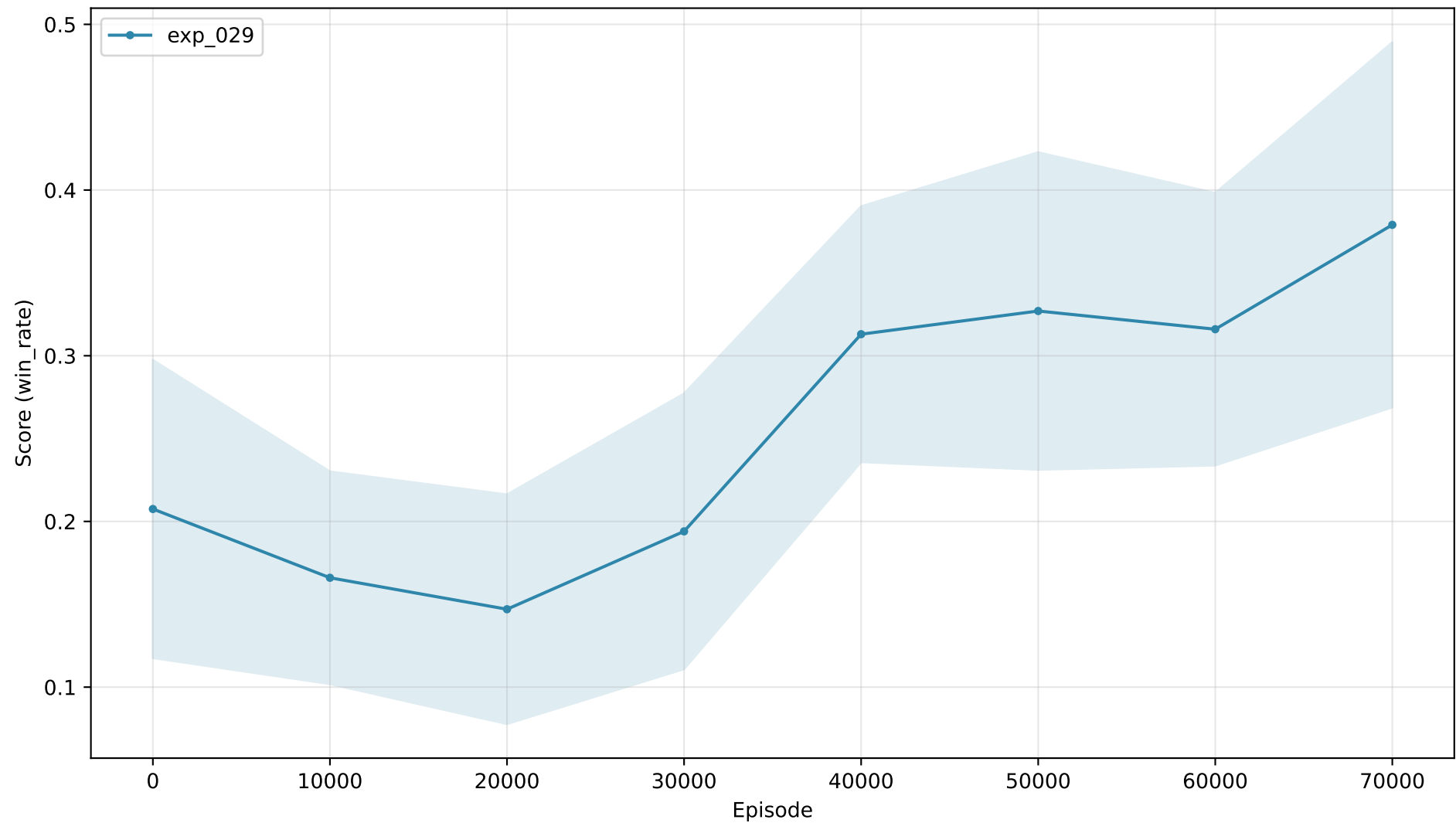
Win Rate vs Fast Minimax
