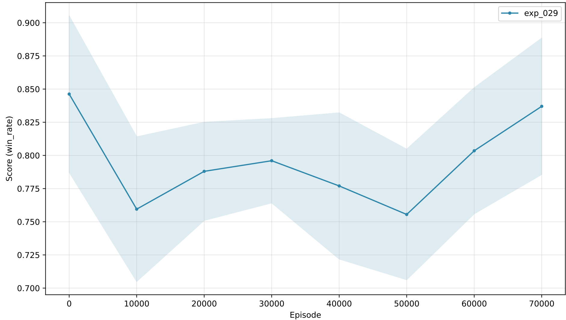
Win Rate vs Greedy
