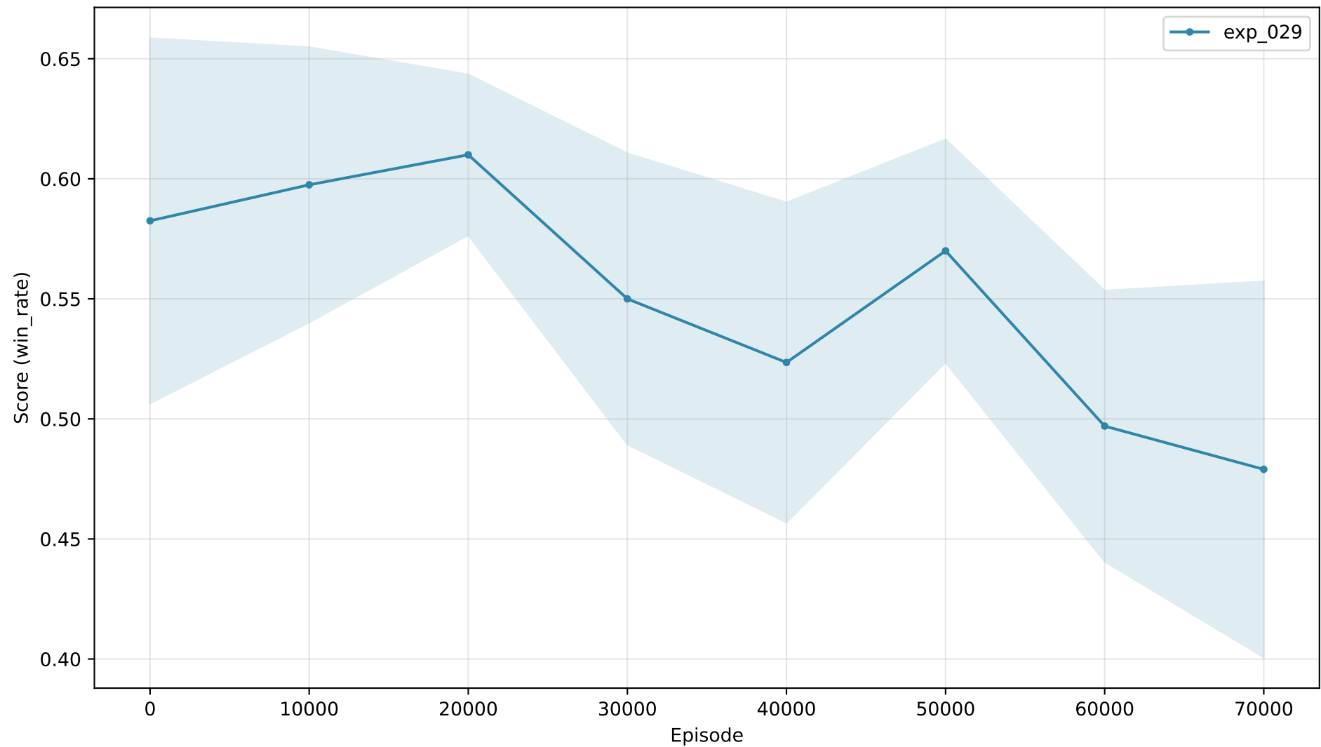
Win Rate vs Heuristic
