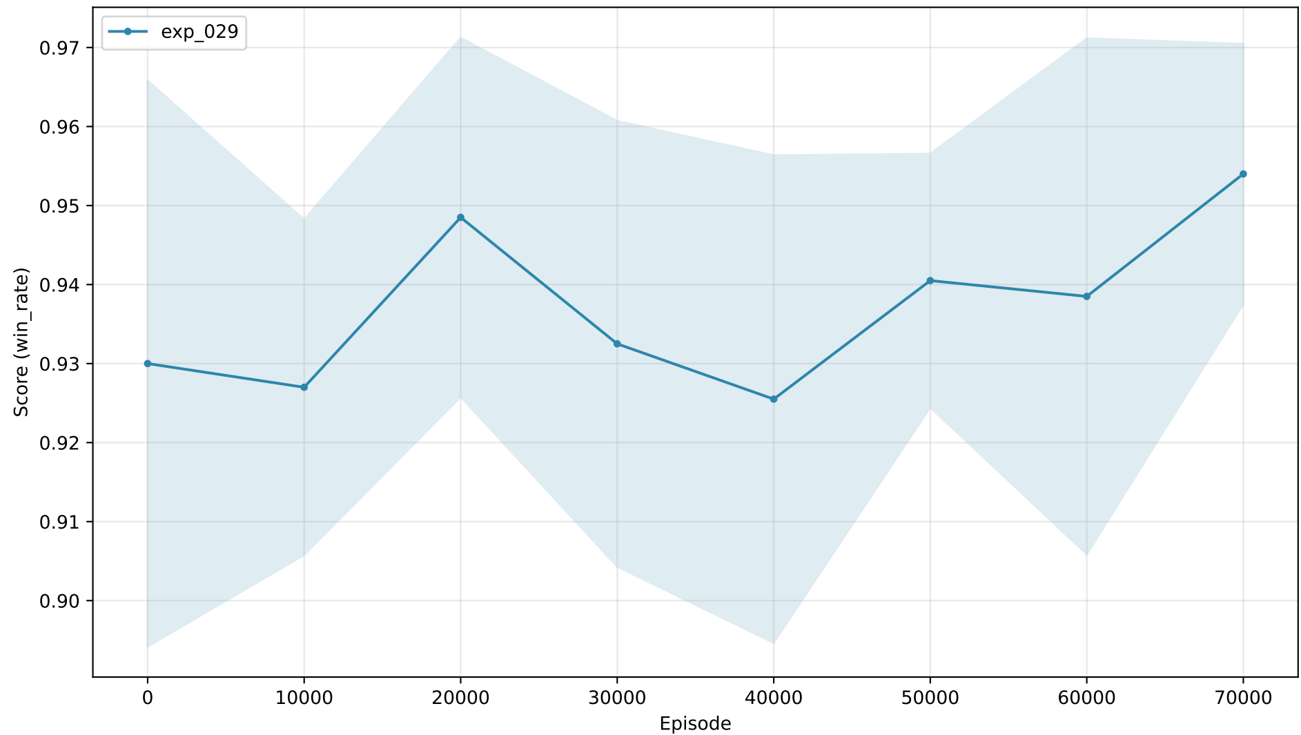
Win Rate vs Random
