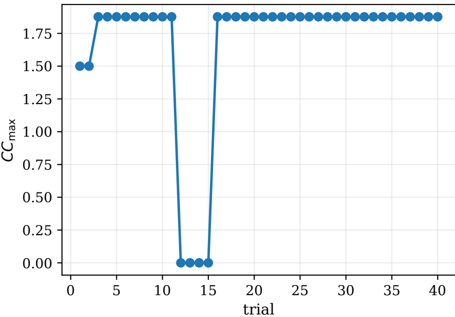
CC_{\max} convergence
