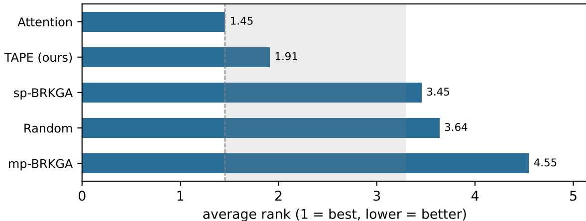
Average HV rank over 11 instances (Nemenyi CD = 1.84)
