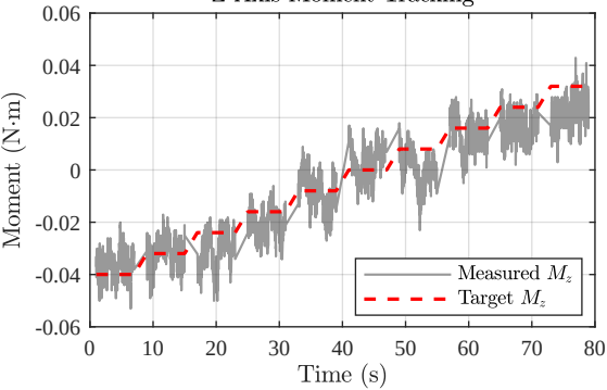
Z-Axis Moment Tracking
