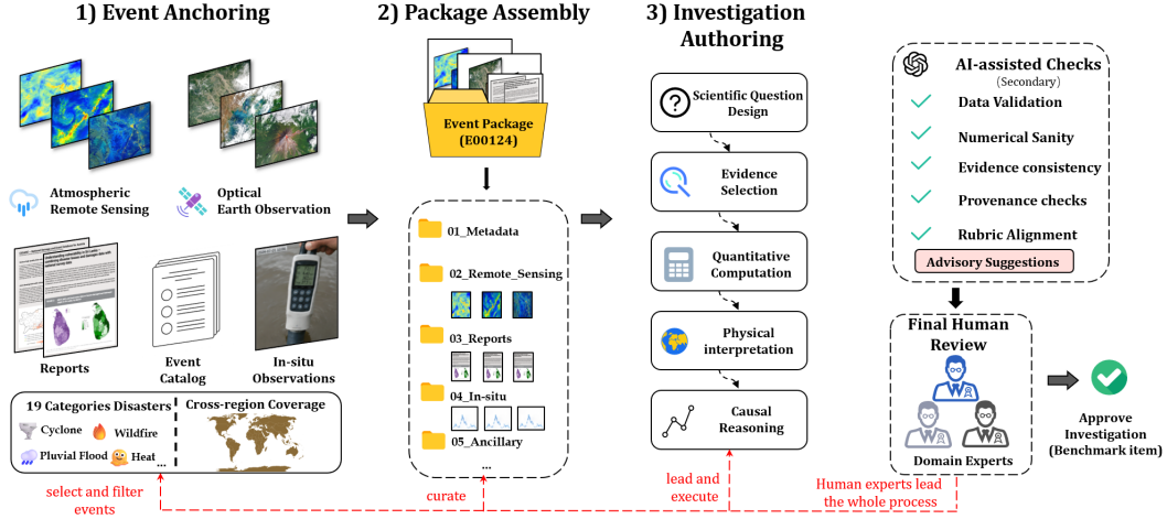
Figure 4: Benchmark construction. Event anchoring, package assembly, task authoring, automated checks, and expert review.
