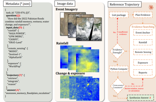
Figure 3: Task interface. Metadata, observations, and an auditable research trajectory.
