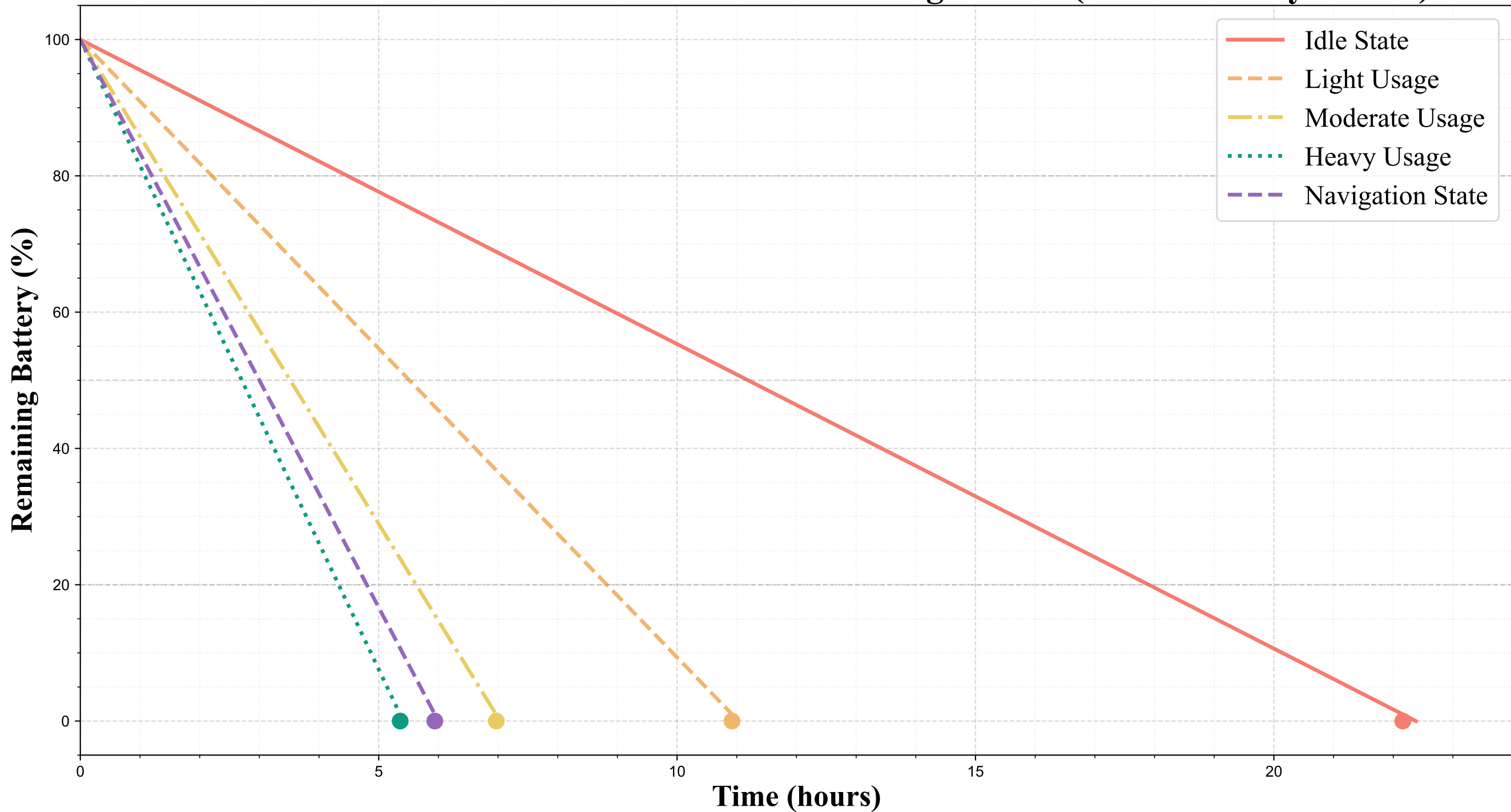
Variation of SOC with Time Under Different Usage States (Initial Battery: 100%)
