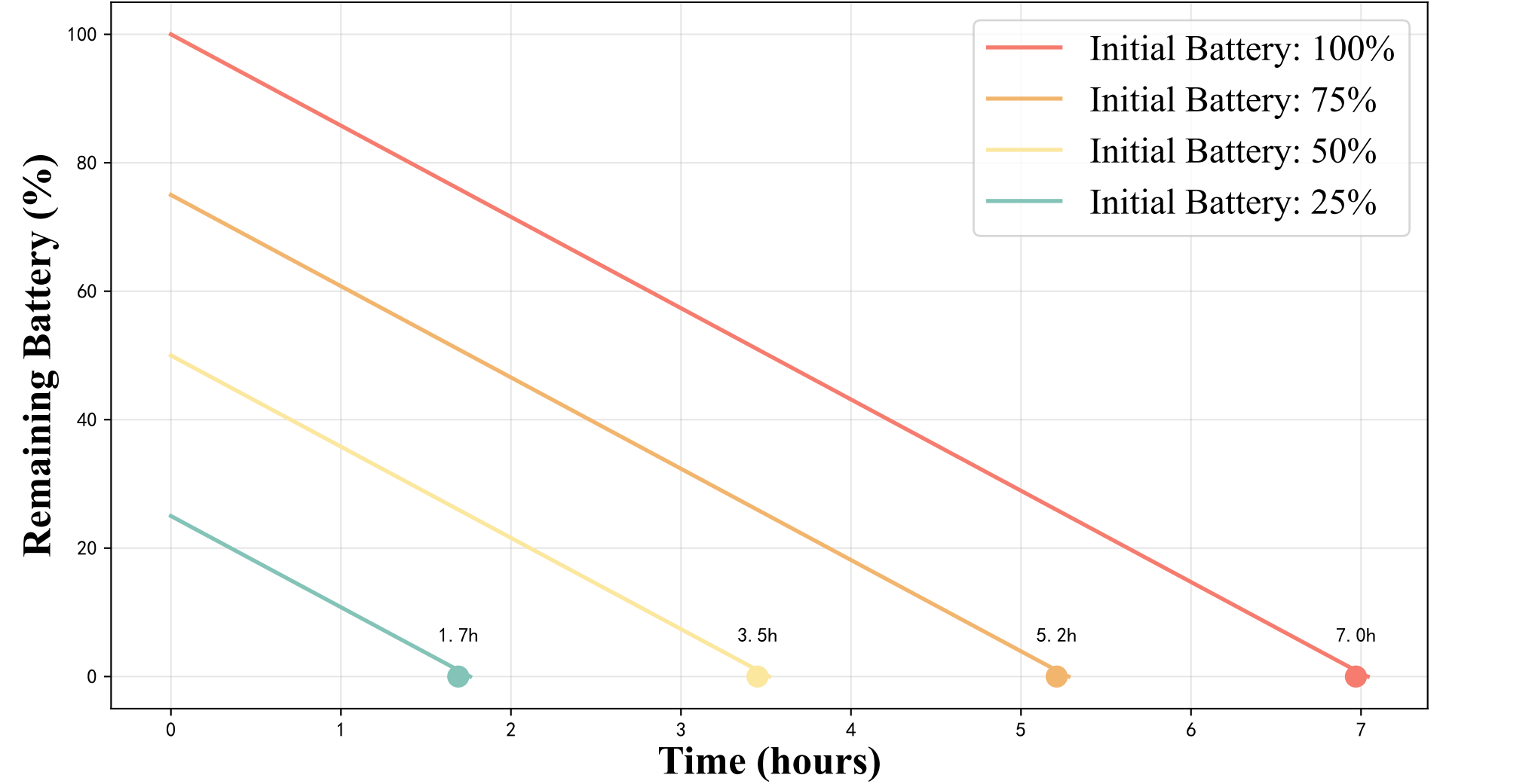
Variation of SOC with Time for Different Initial Battery Levels (Moderate Usage)
