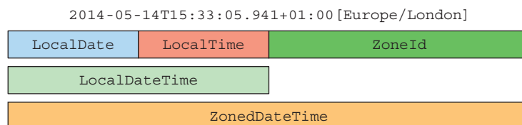
Figure 12.1 Making sense of a ZonedDateTime
