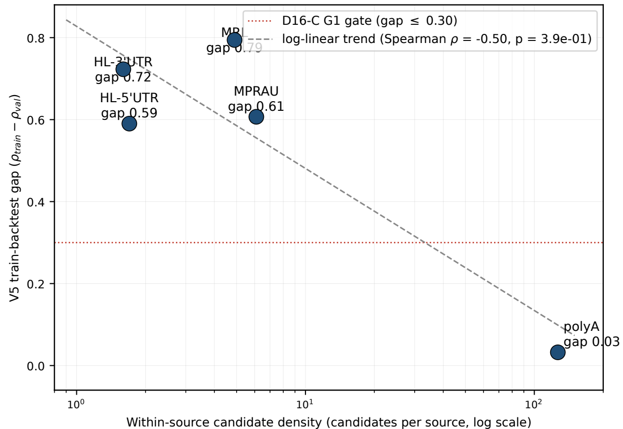
(b) Memorization (train-val gap) follows the same regime
