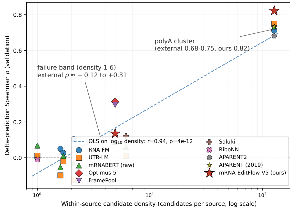
(a) Frozen- \Delta performance vs data regime (n = 25 model-task rows)
