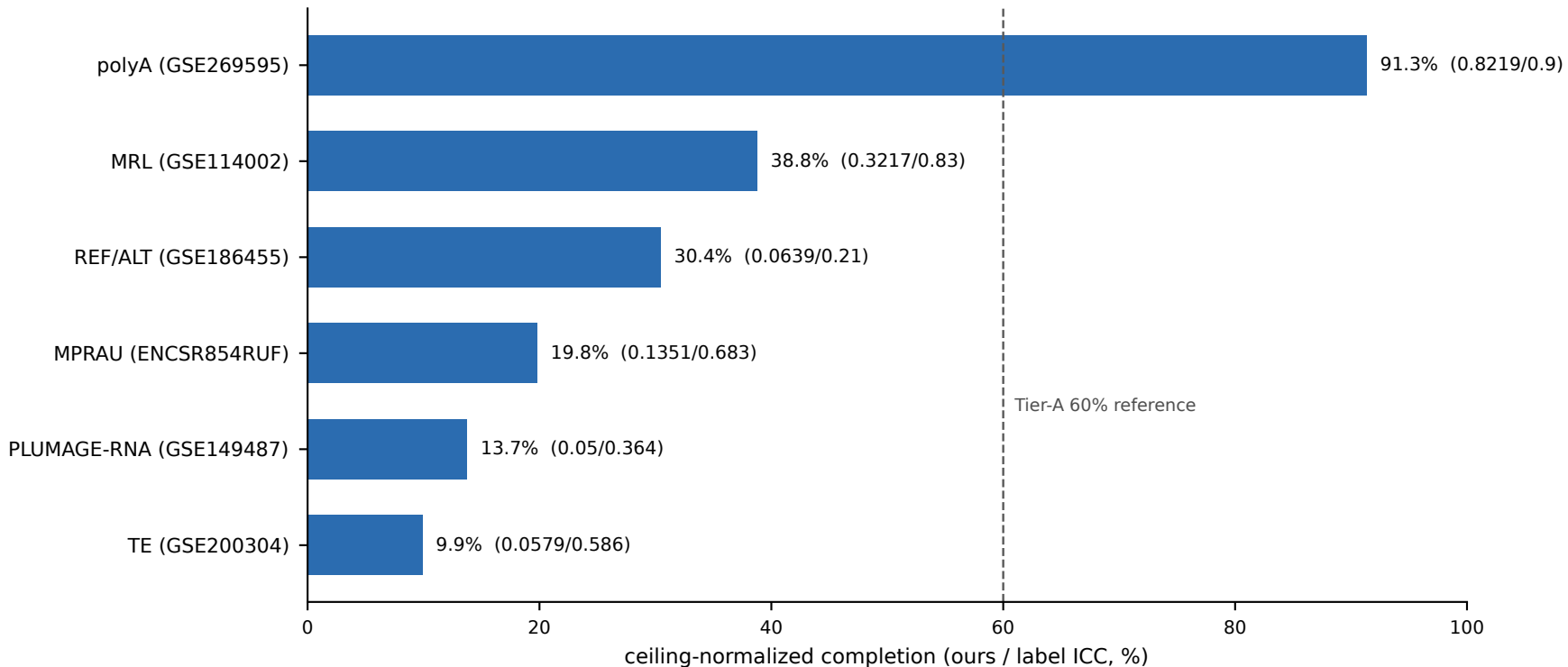
DeltaBench learnability map: label-ceiling completion by task (VALIDATION; ours = best in-house row; ICC = split-half / meta-analytic label reliability)
