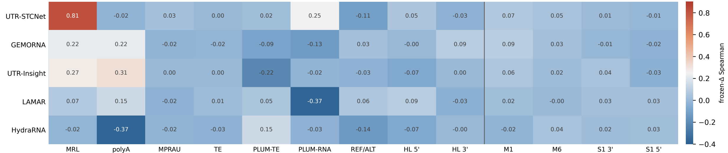
DeltaBench matrix: 5 ported families × 13 tasks (65/65 re-checked)
