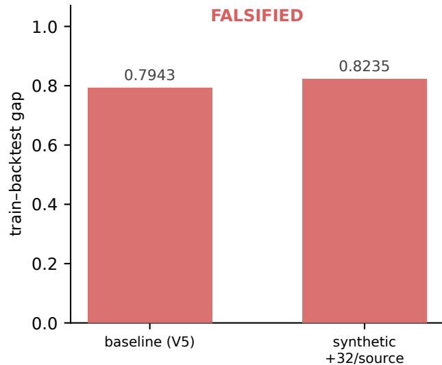
Synthetic density (D16-C)
