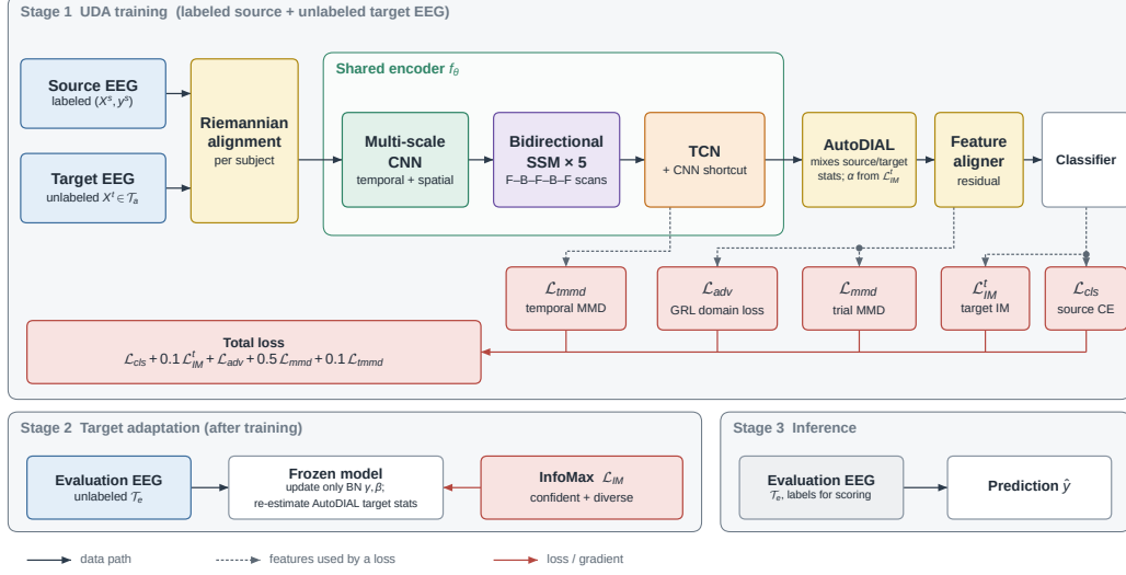
Figure 1: Overview of the framework: training with labeled source and unlabeled target EEG (Stage 1), label-free test-time adaptation on the unlabeled evaluation sessions \mathcal{T}_e (Stage 2), and prediction (Stage 3).
