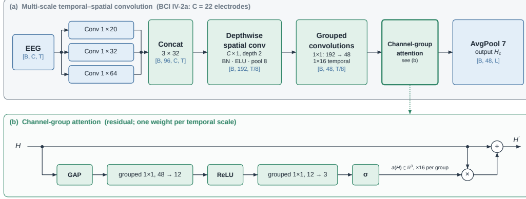
Figure 2: Multi-scale temporal-spatial front-end. (a) Three temporal branches, depthwise electrode filtering, grouped refinement, and channel-group attention produce H_c . (b) Channel-group attention: grouped 1 \times 1 squeeze-excitation yields one sigmoid weight per temporal scale, which rescales that scale’s 16 channels and is added residually.
