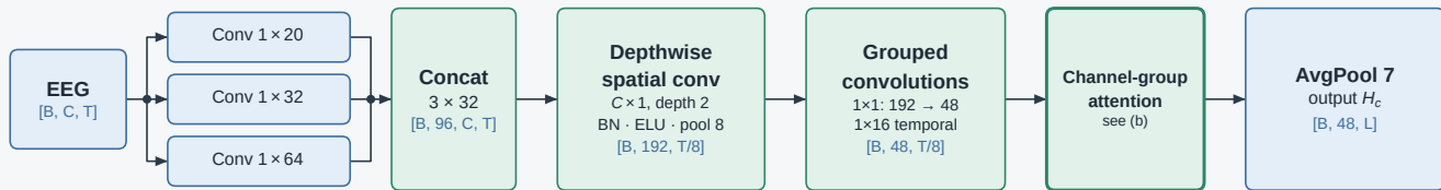
(a) Multi-scale temporal-spatial convolution (BCI IV-2a: C = 22 electrodes)
