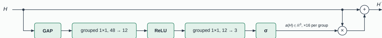
(b) Channel-group attention (residual; one weight per temporal scale)
