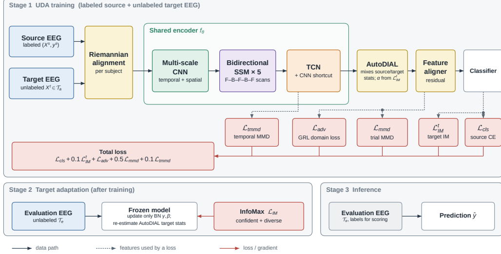
Figure 1: Framework for one LOSO fold: joint source classification and target adaptation with AutoDIAL feature normalization (Stage 1), label-free IM-TTA followed by AutoDIAL target-statistic re-estimation on the evaluation sessions \mathcal{T}_e (Stage 2), and scoring with previously withheld labels (Stage 3).
