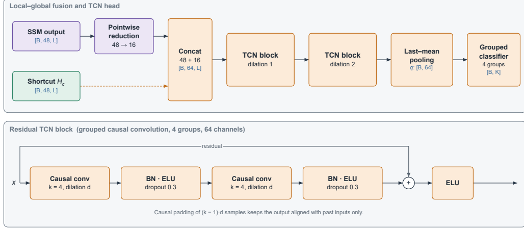
Figure 4: Local-global fusion and TCN head. Top: the reduced SSM output is concatenated with the shortcut H_c and refined by two residual TCN blocks before last-mean pooling and grouped classification. Bottom: structure of one residual TCN block.
