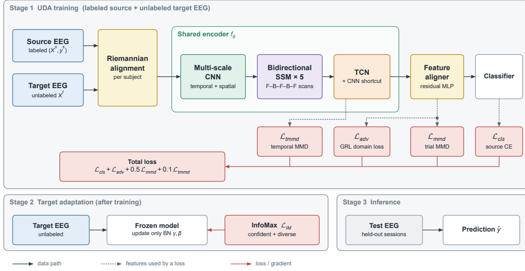
Figure 1: Overview of the proposed framework in one LOSO fold. Stage 1 trains the shared encoder with labeled source EEG and unlabeled target EEG; Stage 2 adapts only BatchNorm parameters on the unlabeled target sessions; Stage 3 evaluates the held-out target sessions.
