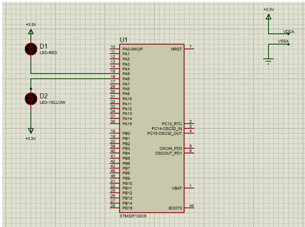
Figure 1: Schematic of Exercise 1 ( https://www.mediafire.com/file/8757v5aae31w504/Ex1.zip/file )
