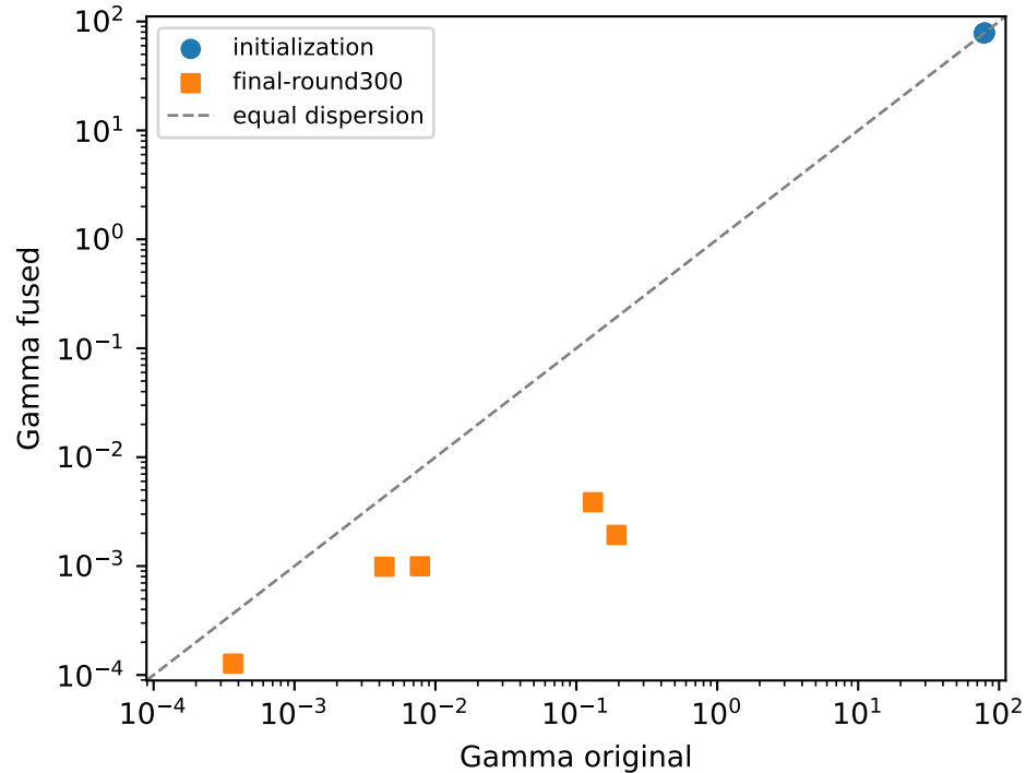
batch-stateless
