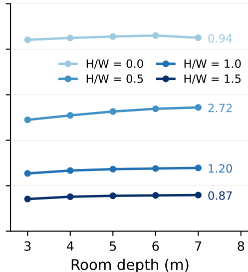
(b) Room depth, all tiers
