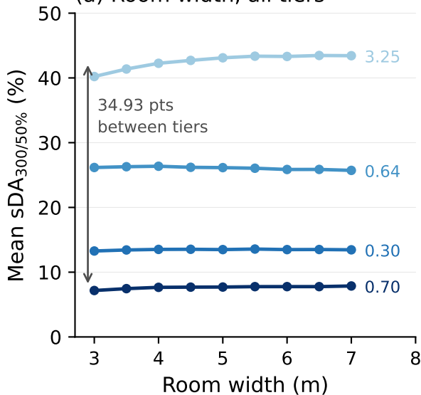
(a) Room width, all tiers
