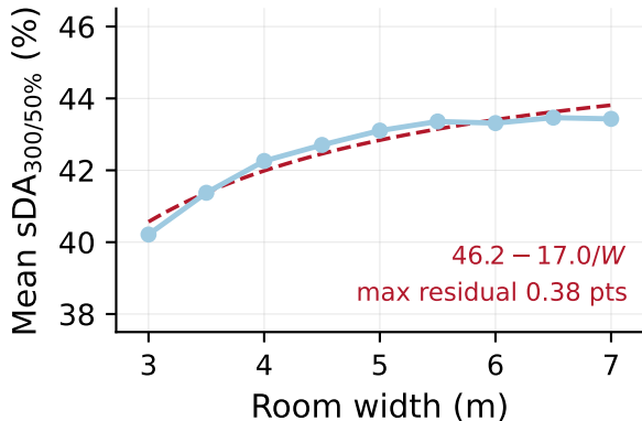
(c) Room width, H/W = 0.0, all orientations
