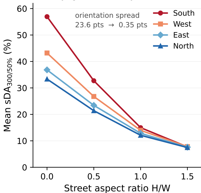
(a) Daylight autonomy
