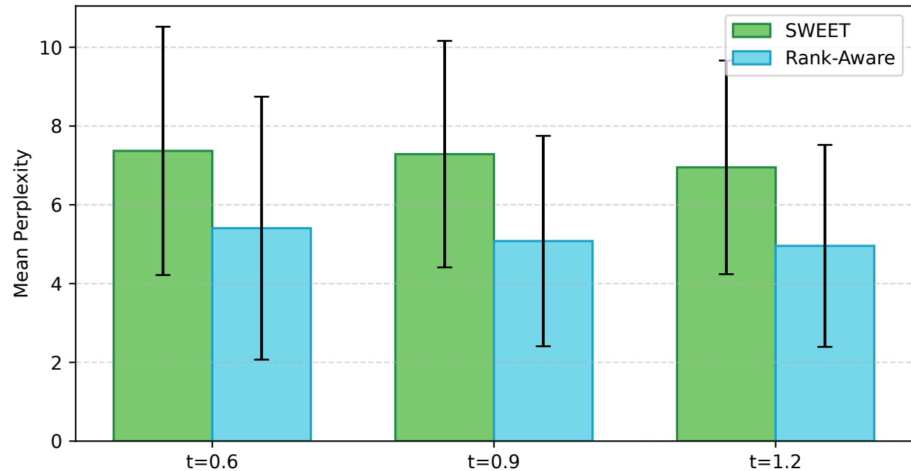
Mean PPL vs Entropy Threshold
